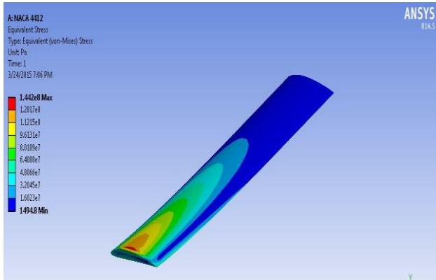
Fig 4: von-mises stress of AA7075
