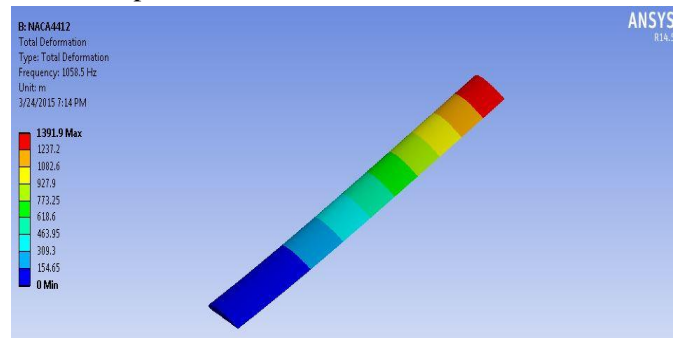
Fig 8: 1 st mode
