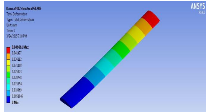
Fig 7: Total deformation of composite aircraft wing
