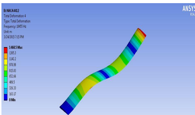
Fig 11: 4th mode
