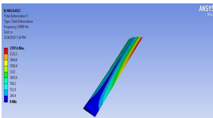
Fig 12: 5th mode
