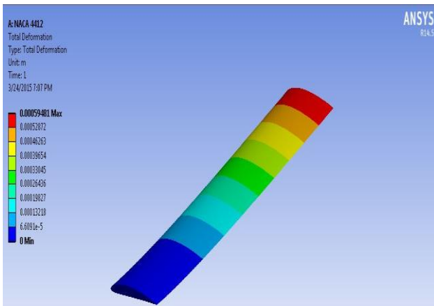
Fig 5: Total deformation of AA7075
