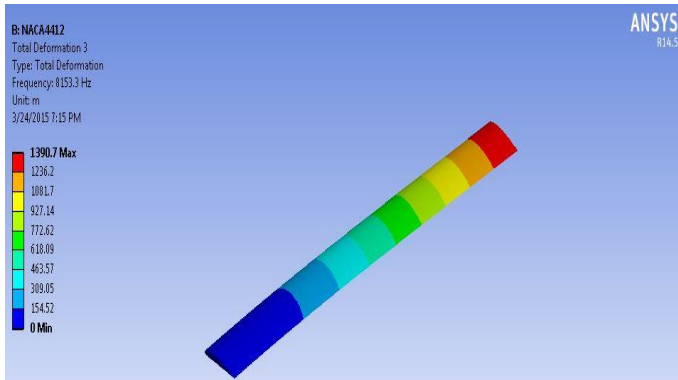
Fig 10: 3rd mode
