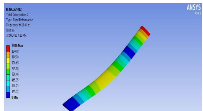
Fig 9: 2nd mode
