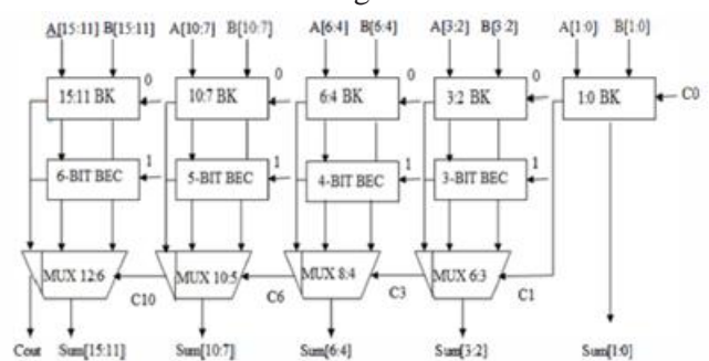
Fig. 7 Block Diagram of 16-bit Modified SQRT BK CSA
