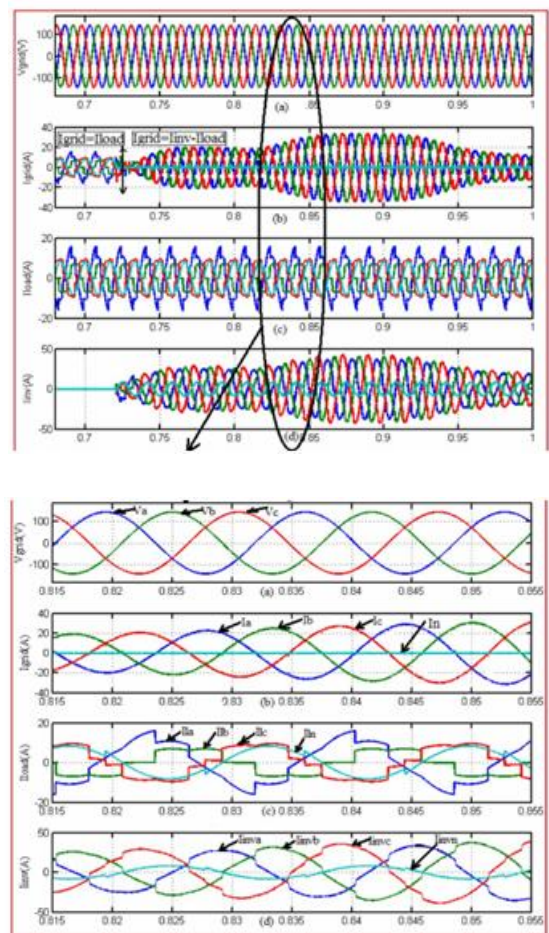
Fig 4. simulation results (a) grid voltages, (b) grid currents, (c) unbalanced load currents and (d) inverter currents.
