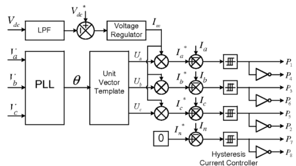
Fig3. Block diagram representation of grid interfacing inverter control
