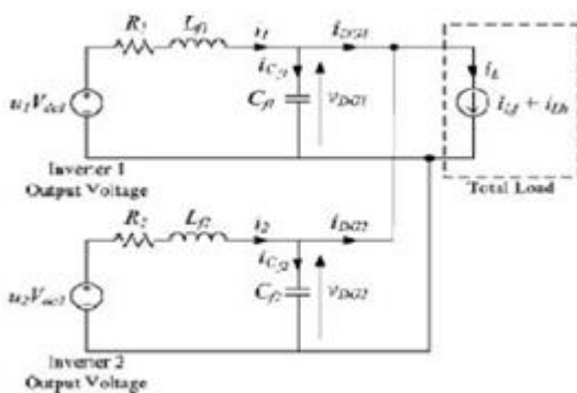
Fig. 5. Equivalent single-phase representation of the DG inverters for islanded operation.
