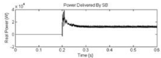
Fig. 21. Real power delivered by SB.
