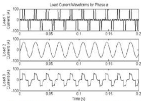
Fig. 9. Per-phase currents drawn by loads 1, 2, and 3.
