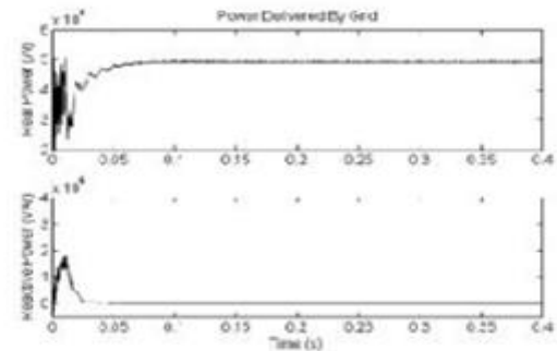
Fig. 16. Real (top) and reactive (bottom) power delivered by the grid.
