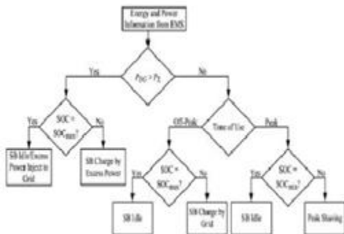
Fig. 2. Operation of the SB during grid-connected operation.
