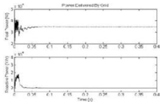
Fig. 18. Real (top) and reactive (bottom) power delivered by the grid.
