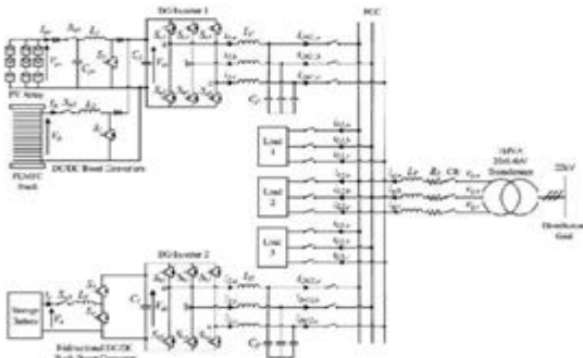
Fig. 1. Overall configuration of the proposed microgrid architecture
