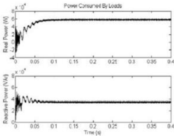
Fig. 14. Real (top) and reactive (bottom) power consumed by loads.
