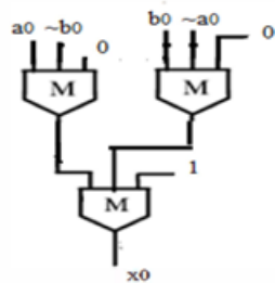
Fig 7.1(b): Modified novel bit adder 1-Calculation of x0
