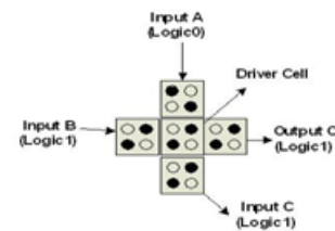
Fig.2 Majority Gate
