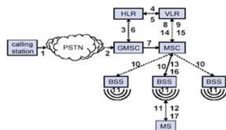
Fig 5.4: operation of GSM on incoming call
