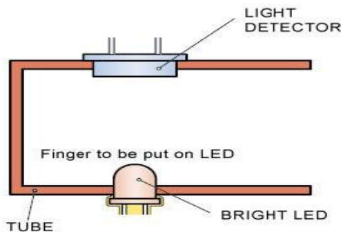
Fig 4.11: sensor construction
