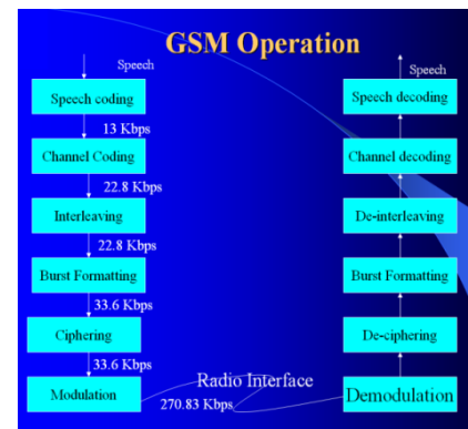
Fig 5.2: Operation of GSM
