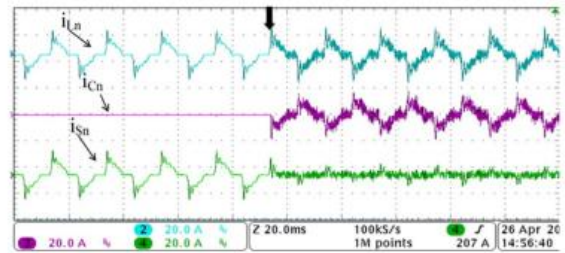
Fig. 10. Experimental results for load neutral ( i_{Ln} ), filter neutral ( i_{Cn} ), and source neutral current ( i_{Sn} ).
