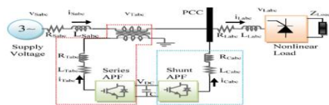
Fig. 1. Basic system configuration of UPQC.
