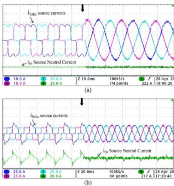
Fig. 9. Experimental results for source current ( i_{Sabc} ) and neutral current ( i_{Sn} ) before and after filter operation in (a) balanced and (b) unbalanced load-current conditions.
