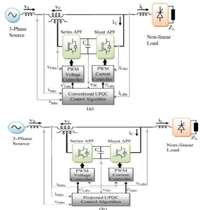
Fig. 4. (a) Conventional and (b) proposed UPQC control block diagrams.
