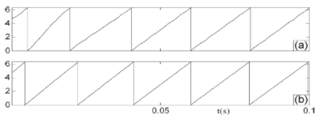
Fig. 3. Transformation angle ( \omega t ) waveforms for the (a) conventional and (b) modified PLL algorithms.
