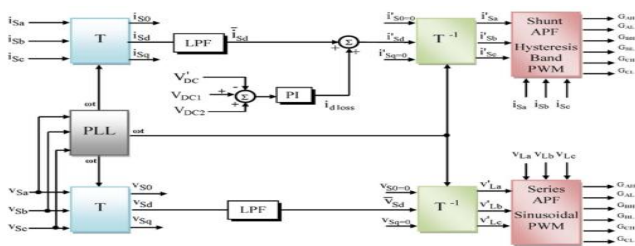
Fig. 5. Proposed SRF-based UPQC control block diagram.
