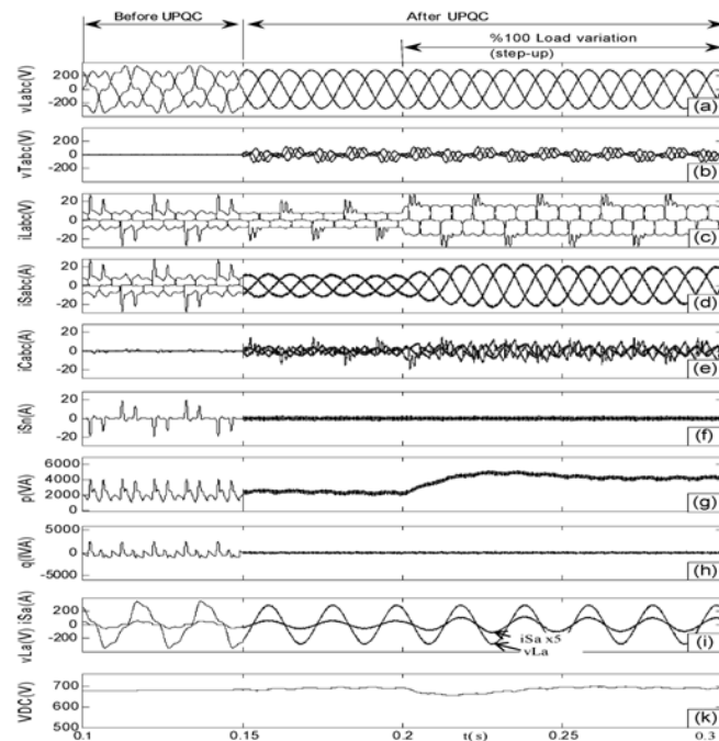
Fig. 7. Simulation results for operational performance of the UPQC system.(a) Load voltages, (b) injected transformer voltages, (c) load currents,(d) source currents, (e) injected compensator currents, (f) source neutral current,(g) instantaneous active power, (h) instantaneous reactive power, (i) load voltage and source current for phase a, and (k) dc-link voltage.
