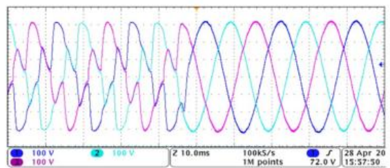
Fig. 11. Experimental results for voltages before and after filter operation in three-phase form at the PCC.
