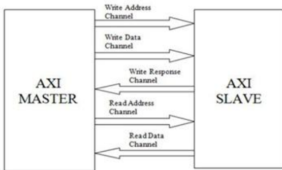
Figure 2 : AXI Master Slave Protocol
