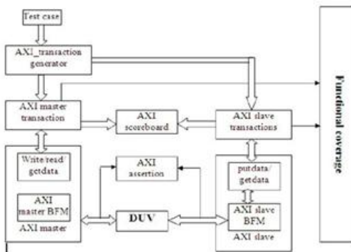
Figure 3 : AXI Verification Environment
