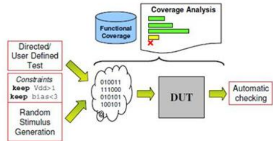
Figure 4: Coverage driven verification flow.
