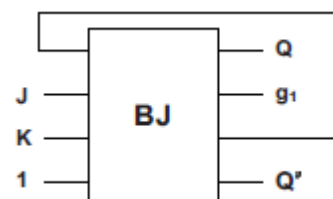
Fig. 3. Proposed Reversible J-K Flip-Flop
