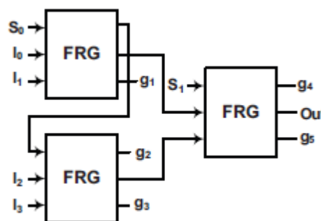
Fig. 4. Proposed Reversible 4-to-1 Multiplexer
