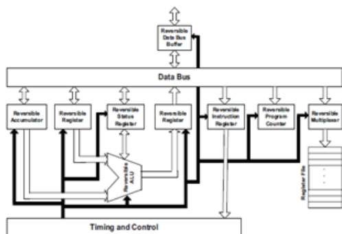
Fig. 1. Outline of the Design of the Proposed Reversible Processor
