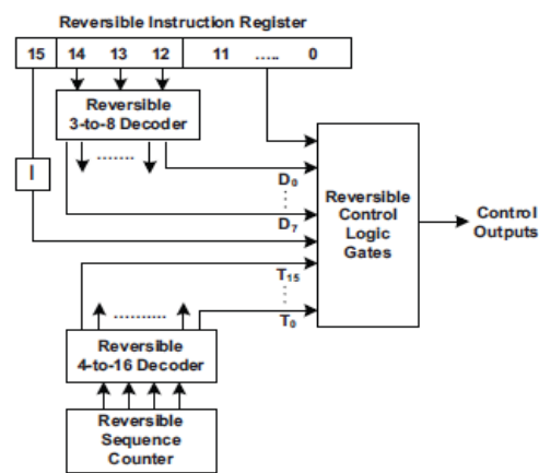
Fig. 6. Proposed Reversible Control Unit
