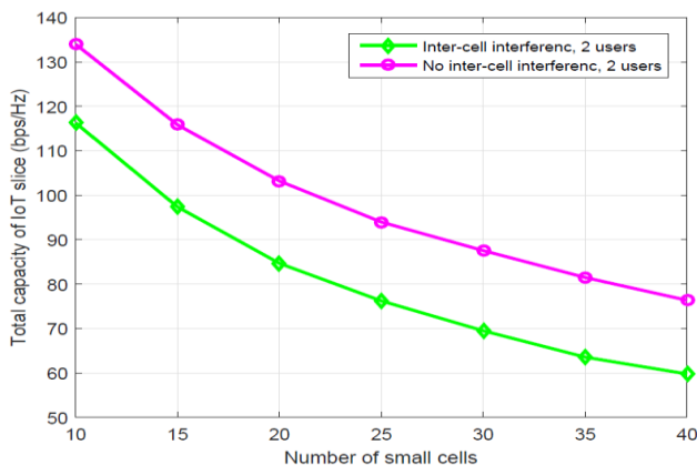
Fig. 6. Total capacity of IoT slice versus the number of small cells.
