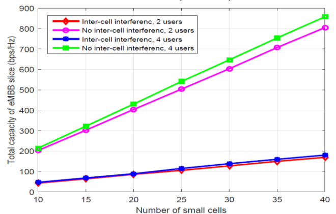
Fig. 4. Total capacity of eMBB slice versus the number of small cells.
