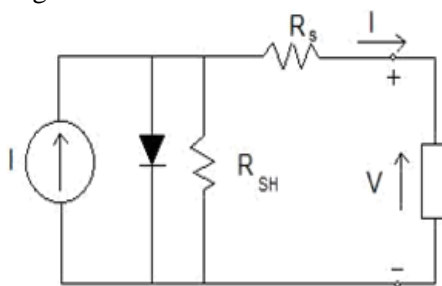
Fig.2 Electrical Equivalent Circuit Model of PV Cell
