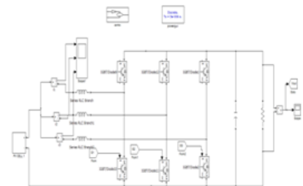
Fig.24 Matlab/Simulink model of proposed converter with PV
