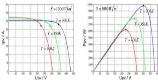
Fig.5 I-V and P-V curve at different temperatures
