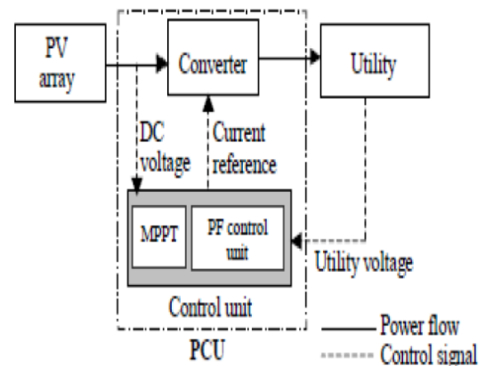
Fig 3 Schematic Diagram of Grid-Connected PV System
