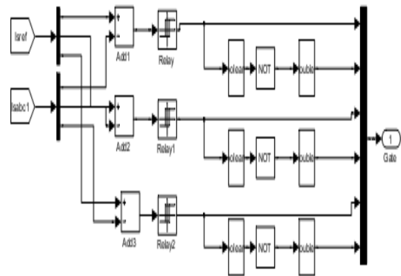
Fig. 4: Simulink Model of Hysteresis Current Control
