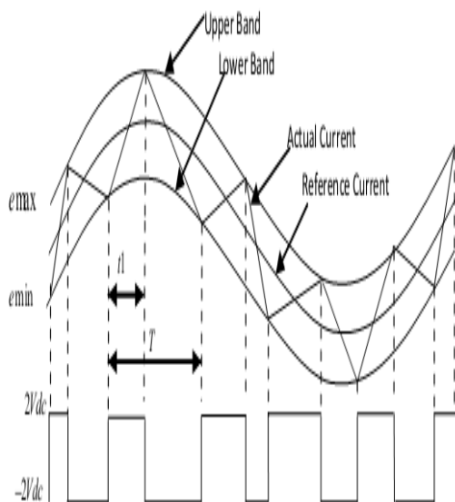
Fig.3: Waveform of Hysteresis current controller
