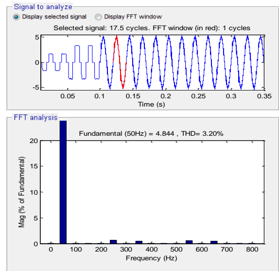
Fig.14: THD of Source Current after Compensation
