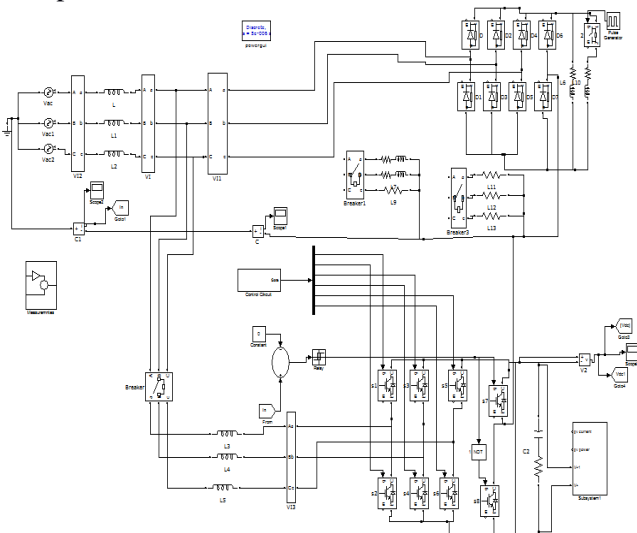
Fig.7: Matlab Implementation
