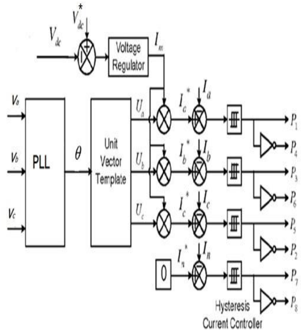
Fig 2: Control scheme
