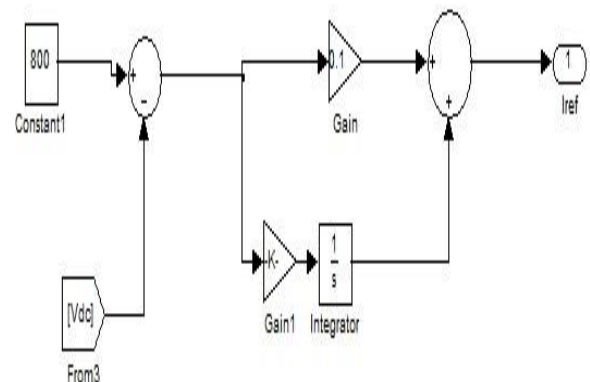
Fig.5: MATLAB Simulink model of PI control
