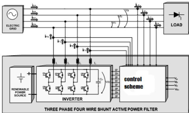
Fig.1: Proposed Three Phase Four Wire System
