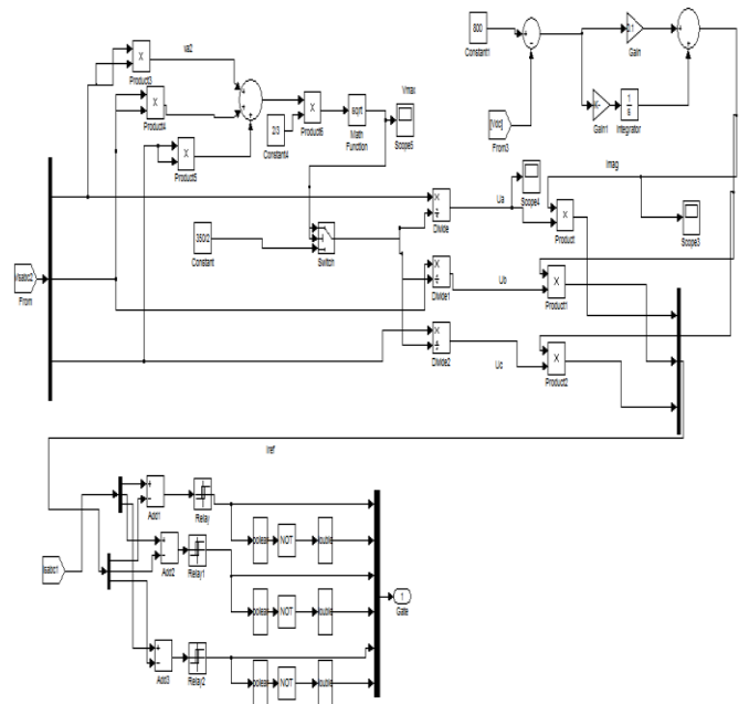
Fig.8: Hysteresis With Pi Controller
