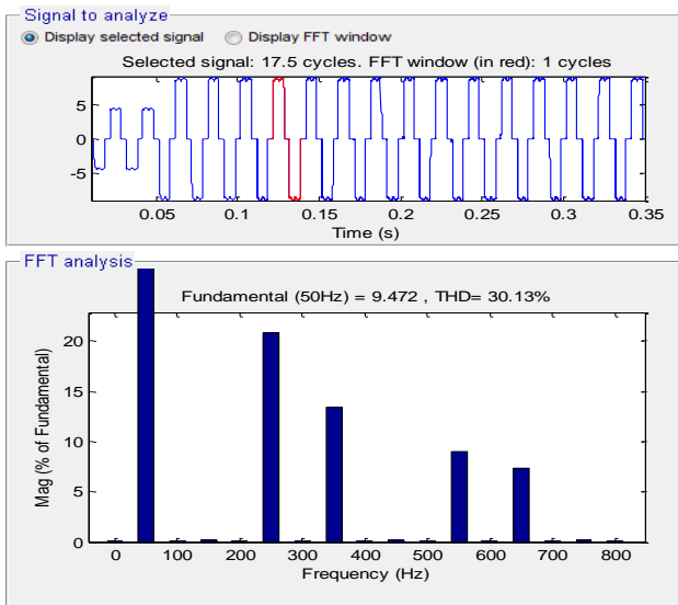
Fig.11: THD of Source Current Before Compensation
