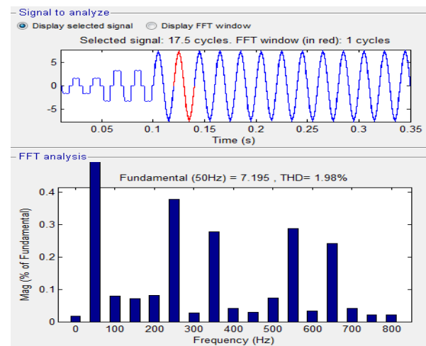
Fig.16: THD of Source Current With fuzzy
