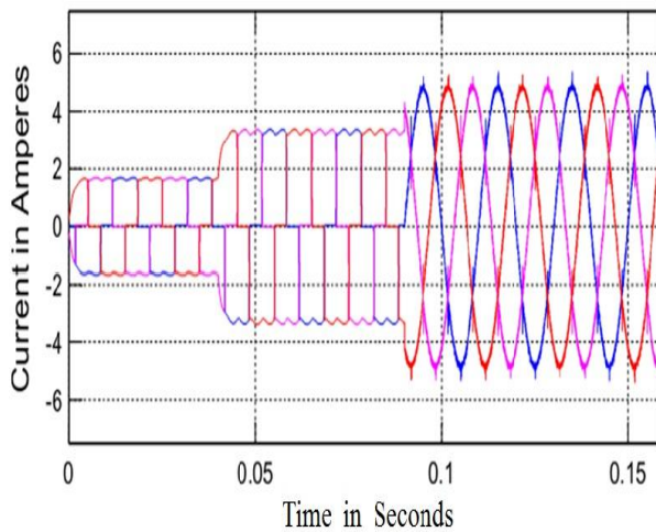
Fig.12: Source Current with Filter
