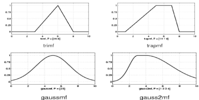
Fig 4 Membership functions
