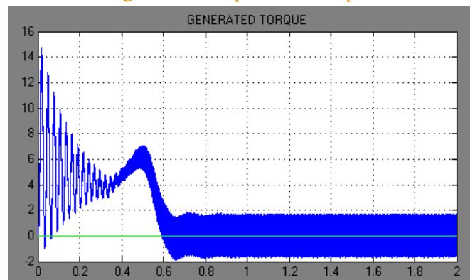
Fig 9 GENERATED TORQUE at no load
