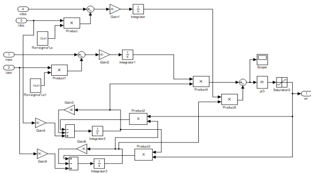
Fig 7 observer design using PI CONTROLLER
