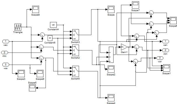
Fig 6 PWM inverter design
