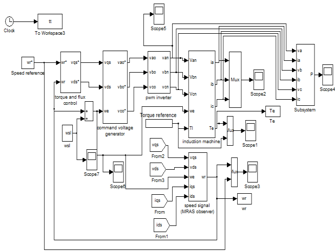
Fig 5 simulation circuit of induction motor using observer
