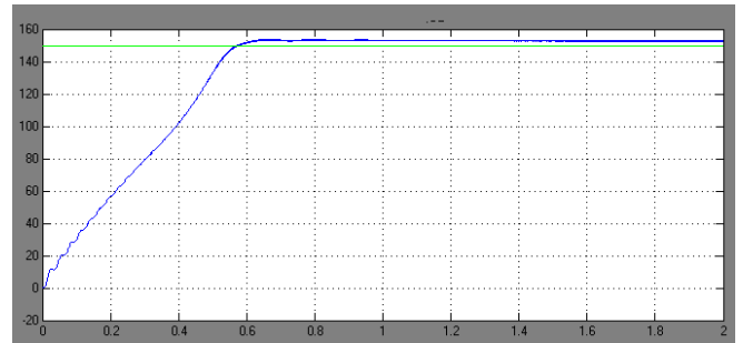
Fig 8 No load speed of 1500 rpm
