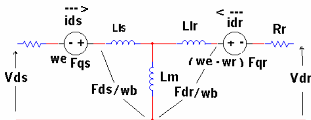
Fig. 1 Dynamic or d-q equivalent circuit of an induction machine at synchronously rotating reference frame.
